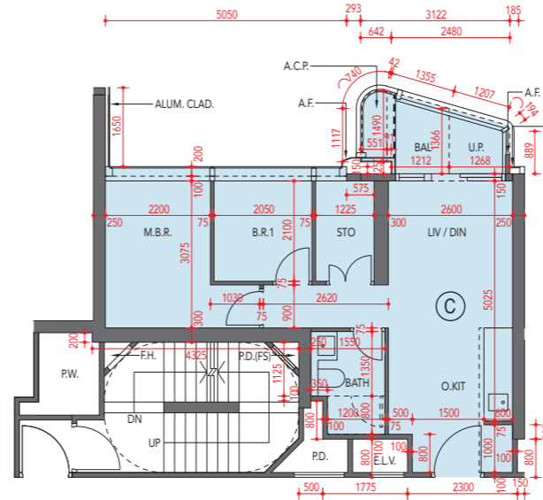
32-35/F Part Plan of Flat C 32-35樓C單位部分平面圖
